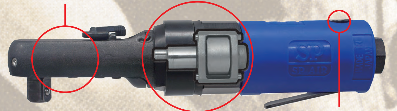
IMPACT MECHANISM [PATENTED] Built-in Power Regulator
